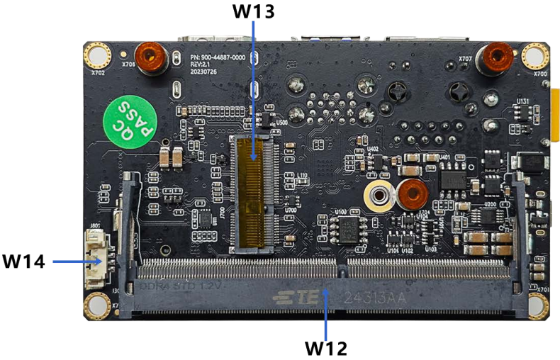
Leetop_A603 V2.1Carrier Board
