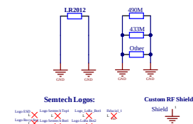
LR20xx IC Frequency band selection:
