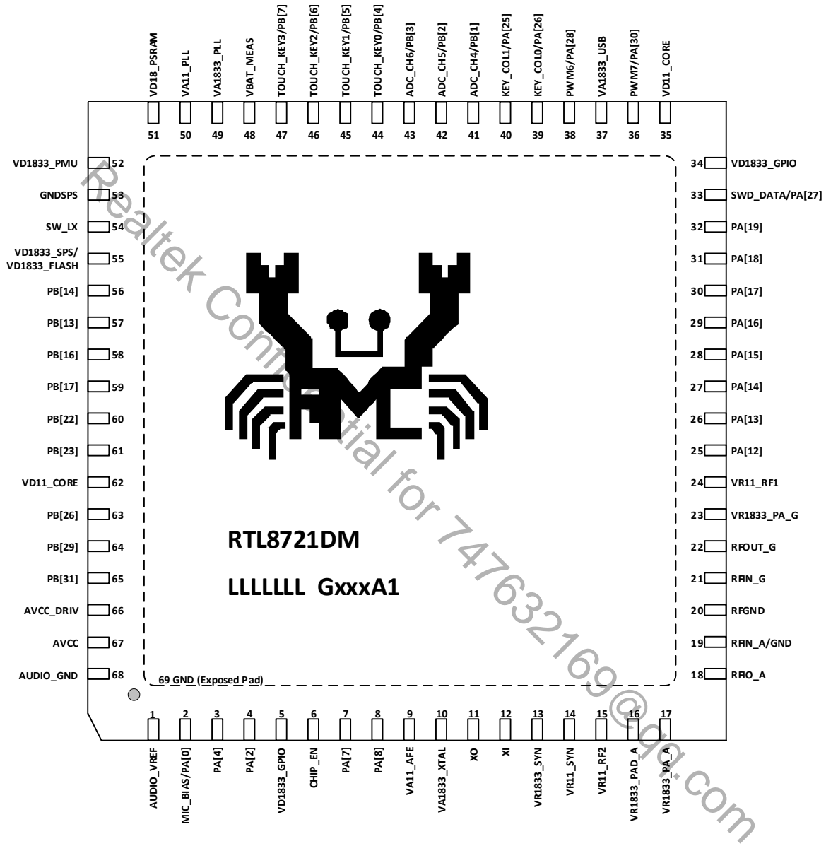
Figure 2-3 QFN68 pin assignment for RTL8721DM
