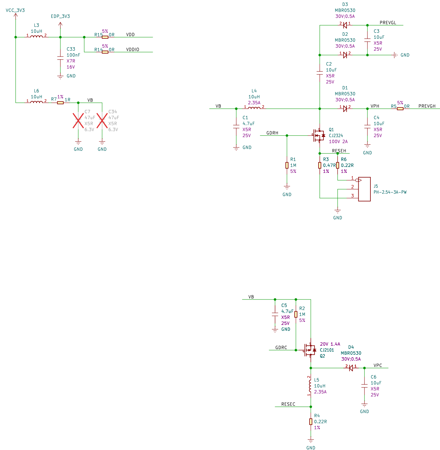
Driver Circuit
