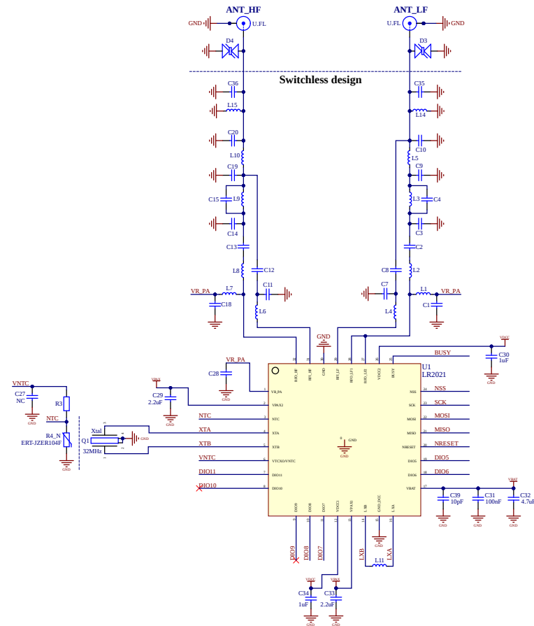
ANT_HF 2.4GHz ANT_LF SubGHz - 868/915MHz
